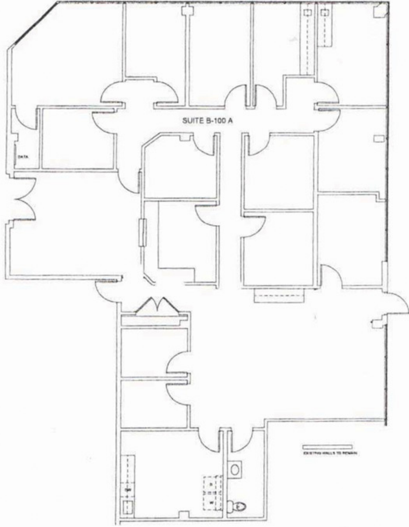
1 NEW FLOOR PLAN BUILDING "B" SUITE B-100 SCALE 1/4" = 1'-0"
